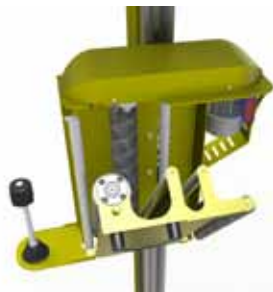
The power pre-stretch carriage offers optimal load containment and optimal film usage. It also allows for easy film threading.
